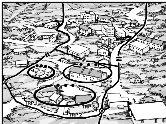
Figure 6-9. Defensive strongpoint.
